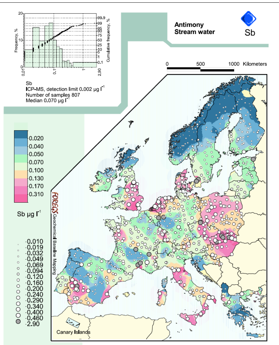
Figure 3-6 FOREG map showing measured concentrations of Sb in European stream water ( http://www.gsf.fi/publ/foregsatlas/maps/Water/w_icpms_sb_edit.pdf ).
