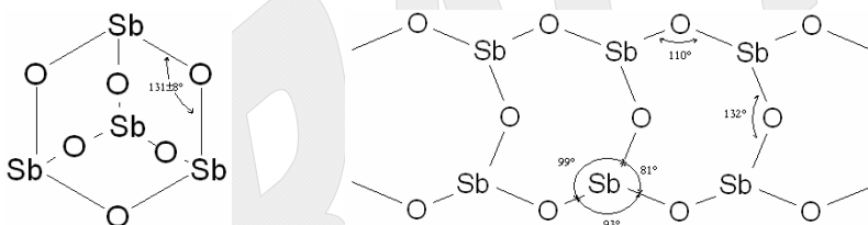
Figure 1-2 Valentinite
