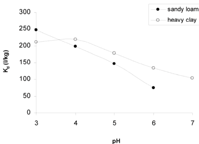
Figure 3-4 Dependence of K_d of antimony (in soils amended with 1000 mg Sb/kg as \text{Sb}_2\text{O}_3 ) on pH for 2 soils. Solution concentrations of antimony were measured in water extracts (S:L = 1/3 kg/l) (Pauwels, 1985) (Reproduced from Degryse and Smolders (2004)).
