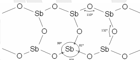
Figure 1-2 Valentinite
