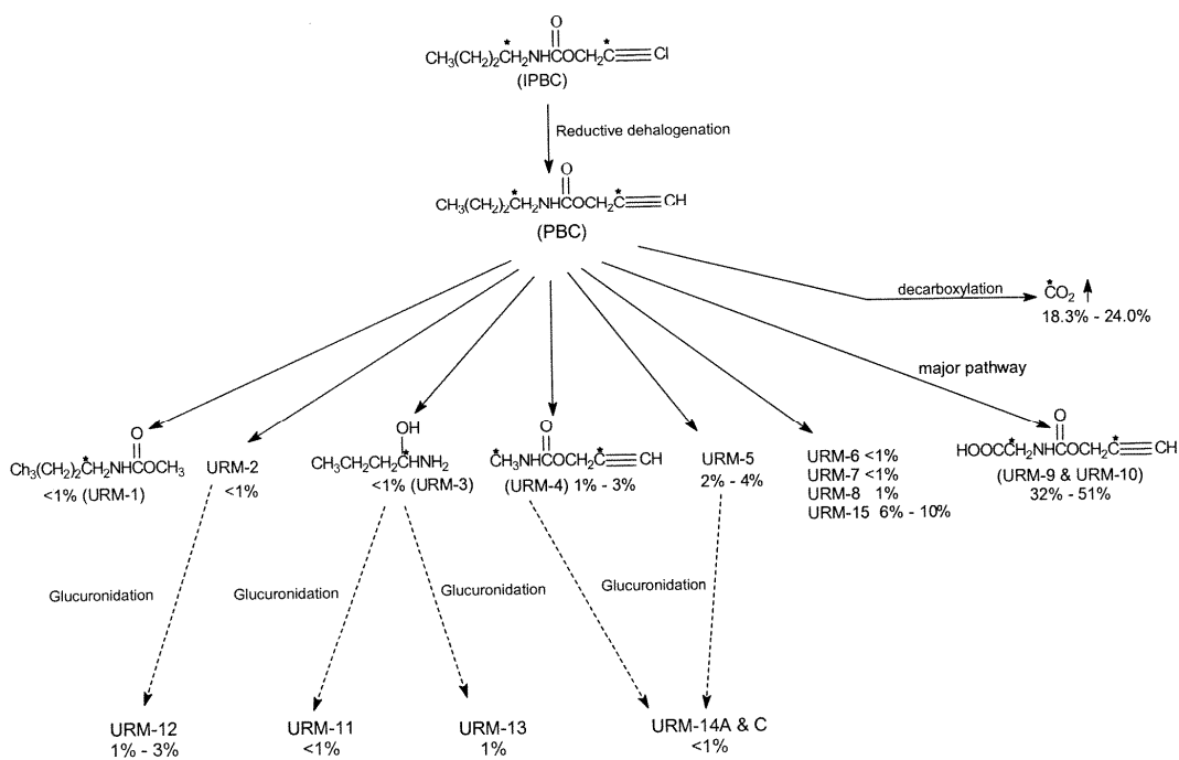
Proposed metabolic pathway of ^{14}\text{C} -IPBC after oral administration (percentages are based on total dose administered)
