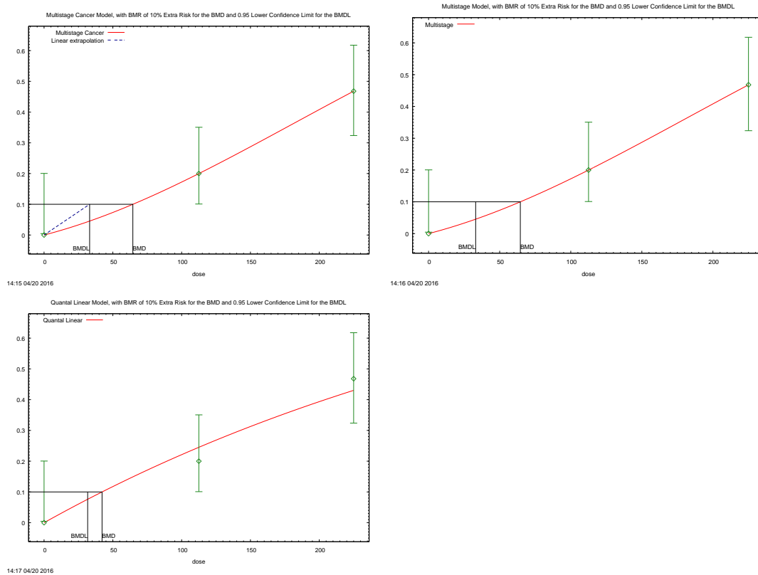
Figure 1: Graphs of the BMD analysis using the different models to fit the data on incidences of transitional-cell carcinoma of the urinary bladder in female rats orally exposed to o -toluidine for 2 years (Table 8) (NCI, 1979)
