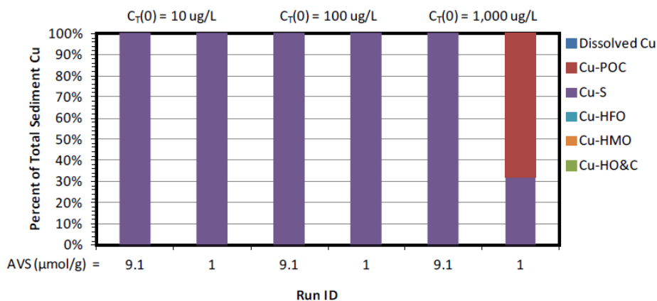
Figure 6. Summary of day 20 sediment copper speciation for initial copper concentrations of 10, 100, and 1,000 μg/L, in oxic sediment
