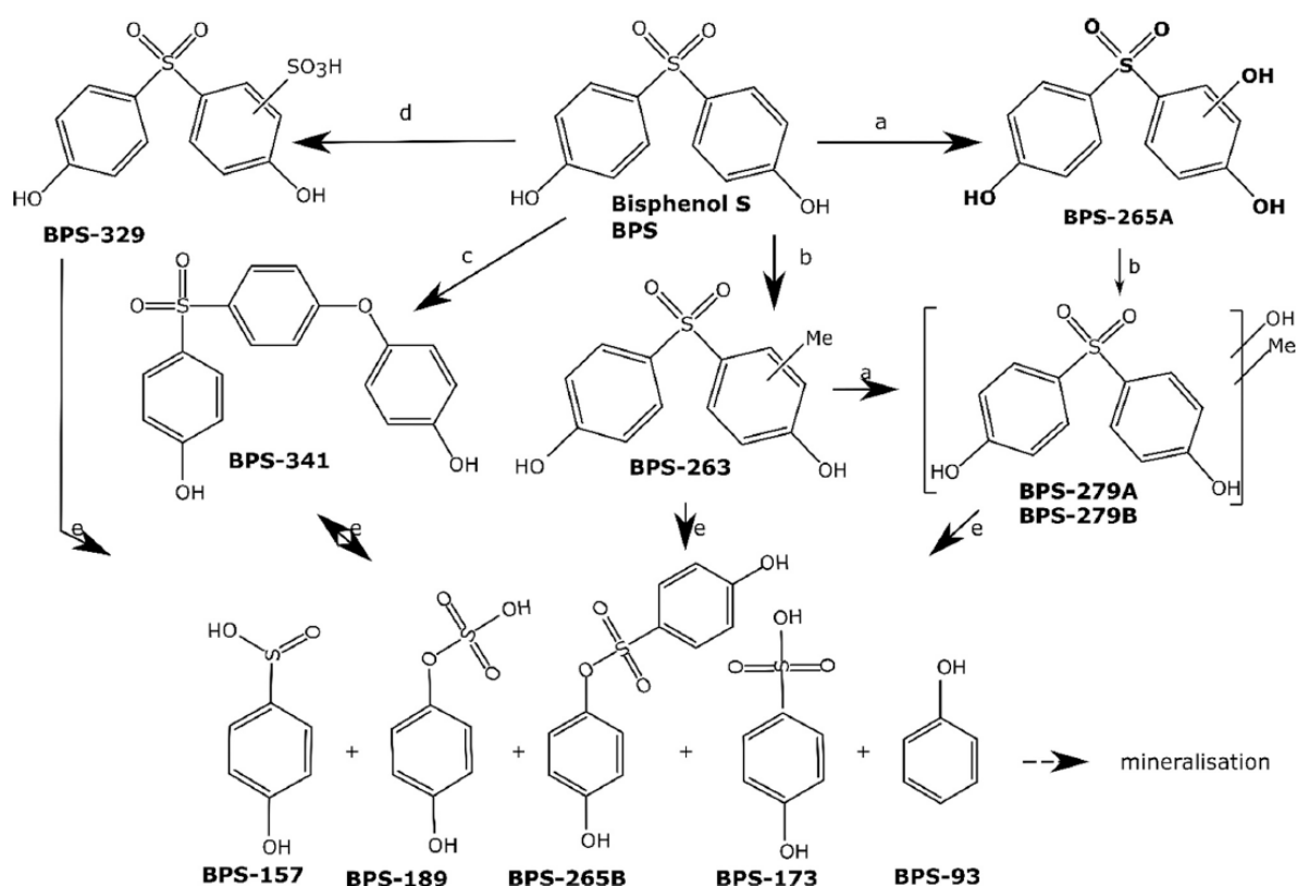
Figure 1: proposed biodegradation pathway of BPS in activated sludge
