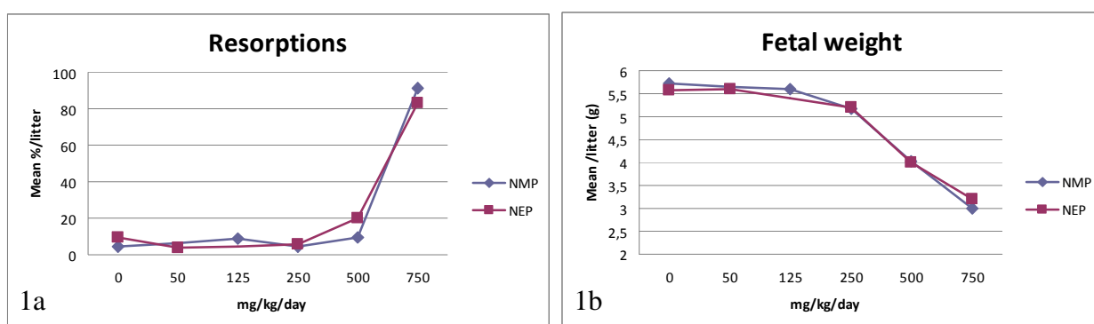
Fig. 1 Comparison of resorptions (1a), reduction of fetal weight (1b) and malformations (1c) induced by NEP in Saillenfait 2007 and by NMP in Saillenfait 2002.
