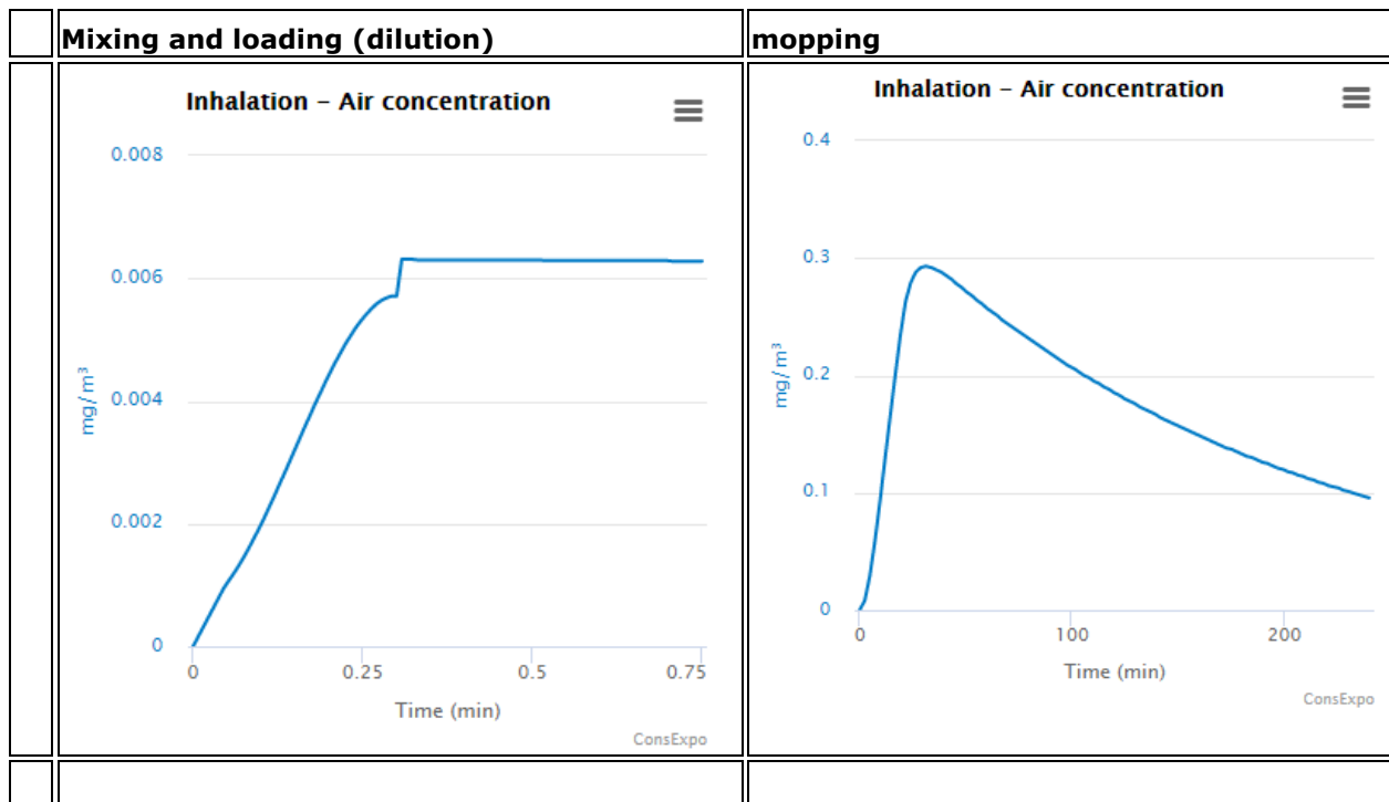
Graph II.3 Formic Acid air concentration during mopping
