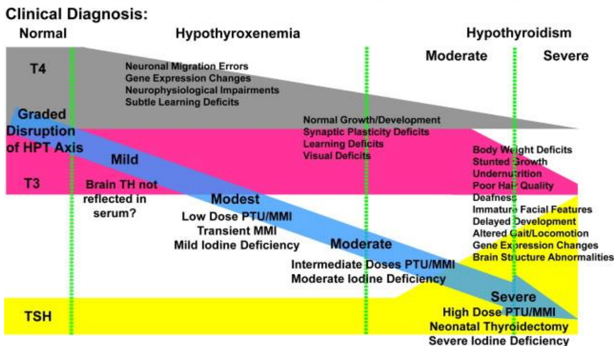
Figure 7: Gradient of thyroid hormone insufficiency.
