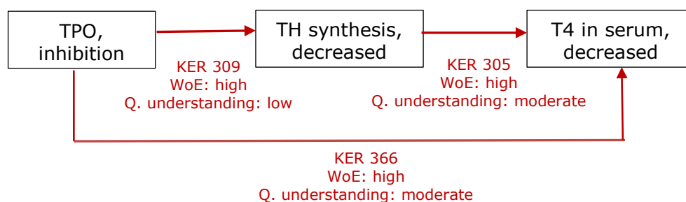
Figure 3: Key events relationships of the endocrine mode of action of TPO inhibition from AOP 42 9 (OECD AOP n°13, Crofton et al. , 2009) (Q=quantitative)
