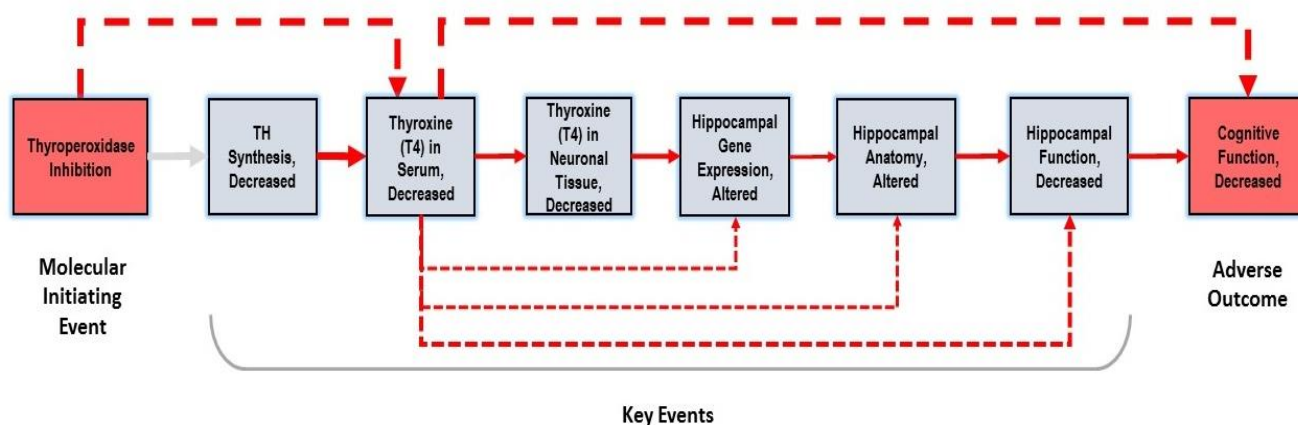
Figure 5: AOP Inhibition of Thyroperoxidase and Subsequent Adverse Neurodevelopmental Outcomes in Mammals
