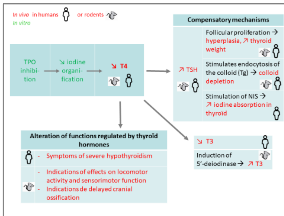
Figure 4: Biological plausible link between findings observed after exposure to resorcinol. Decreased T4 is a direct consequence of inhibition of TH synthesis resulting from TPO inhibition. Modification of the MIT/DIT ratio also indicates that the organification process leading to TH synthesis is disturbed.
