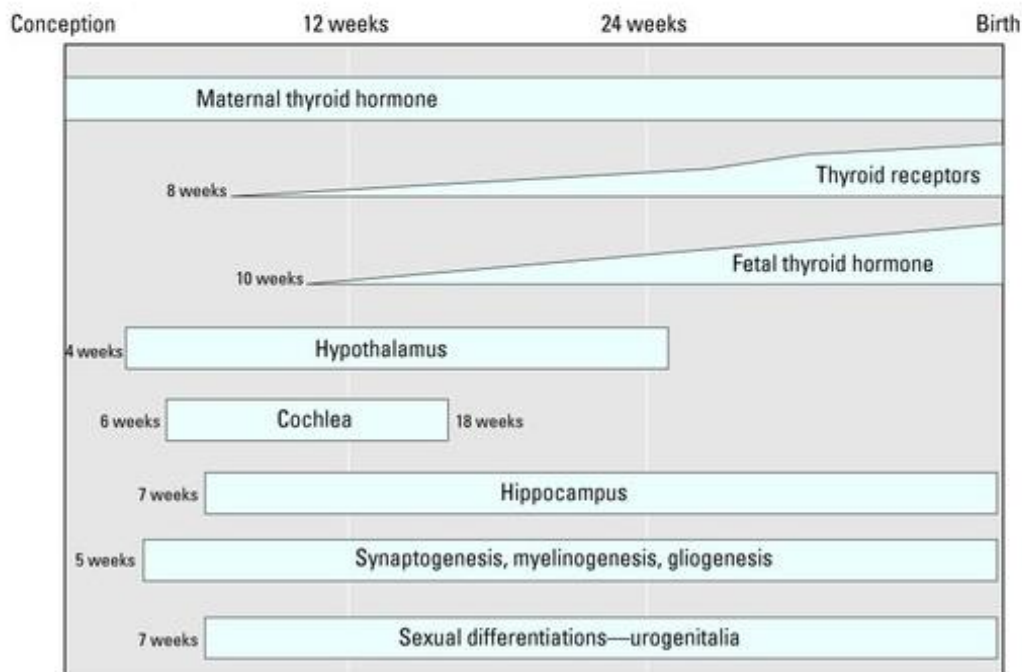
Figure 6: Role of thyroid hormones in foetal neurologic development in relation to timing of several landmark stages of development in humans. (From Colborn (2004), adapted from Howdeshell (2002)).
