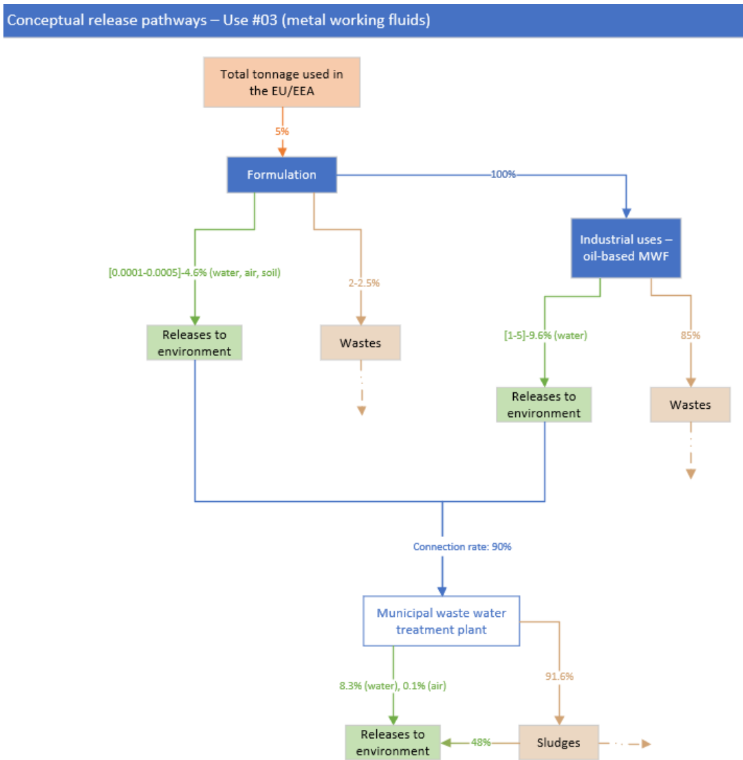
Figure 7: Conceptual release pathways – Use#03 (metalworking fluids)
